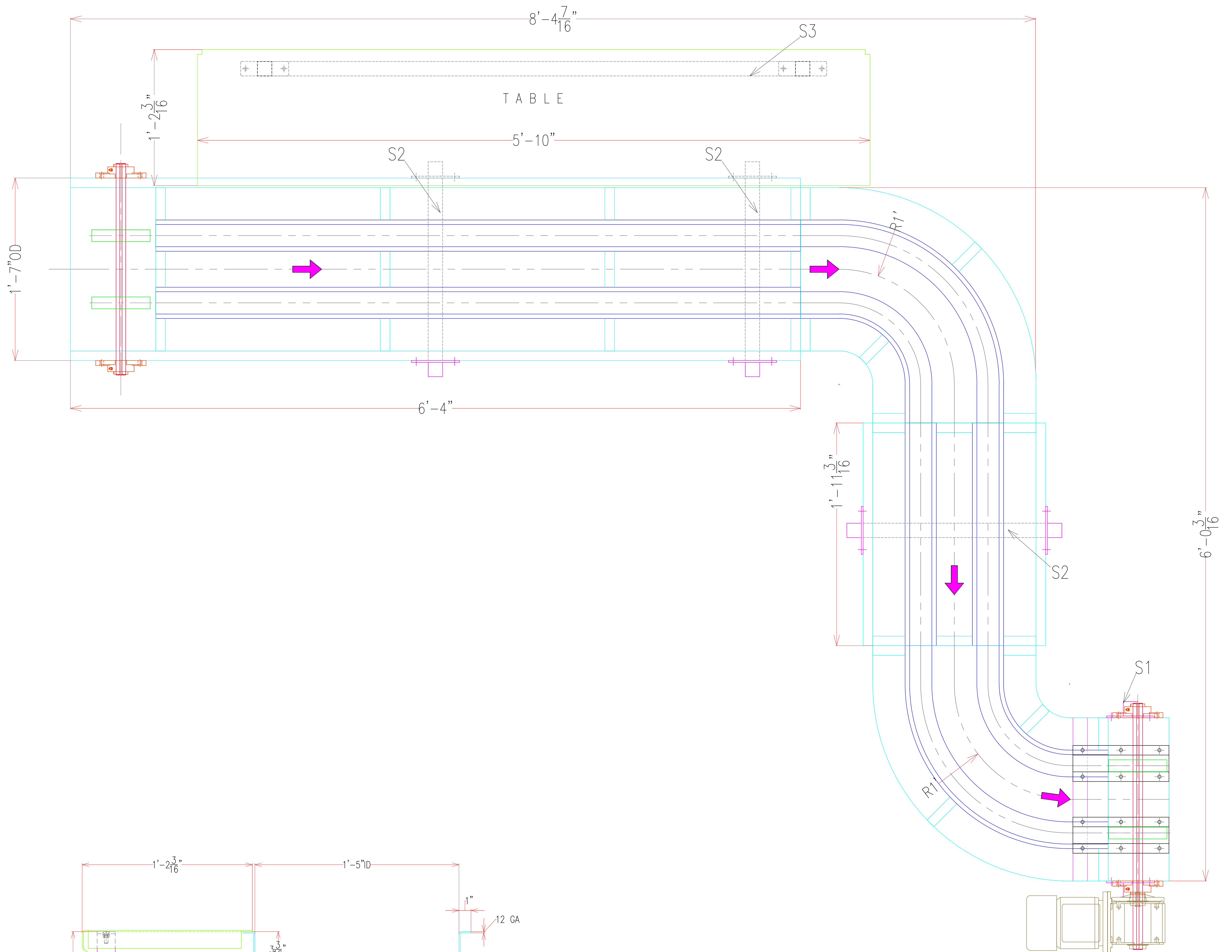
TOP VIEW
