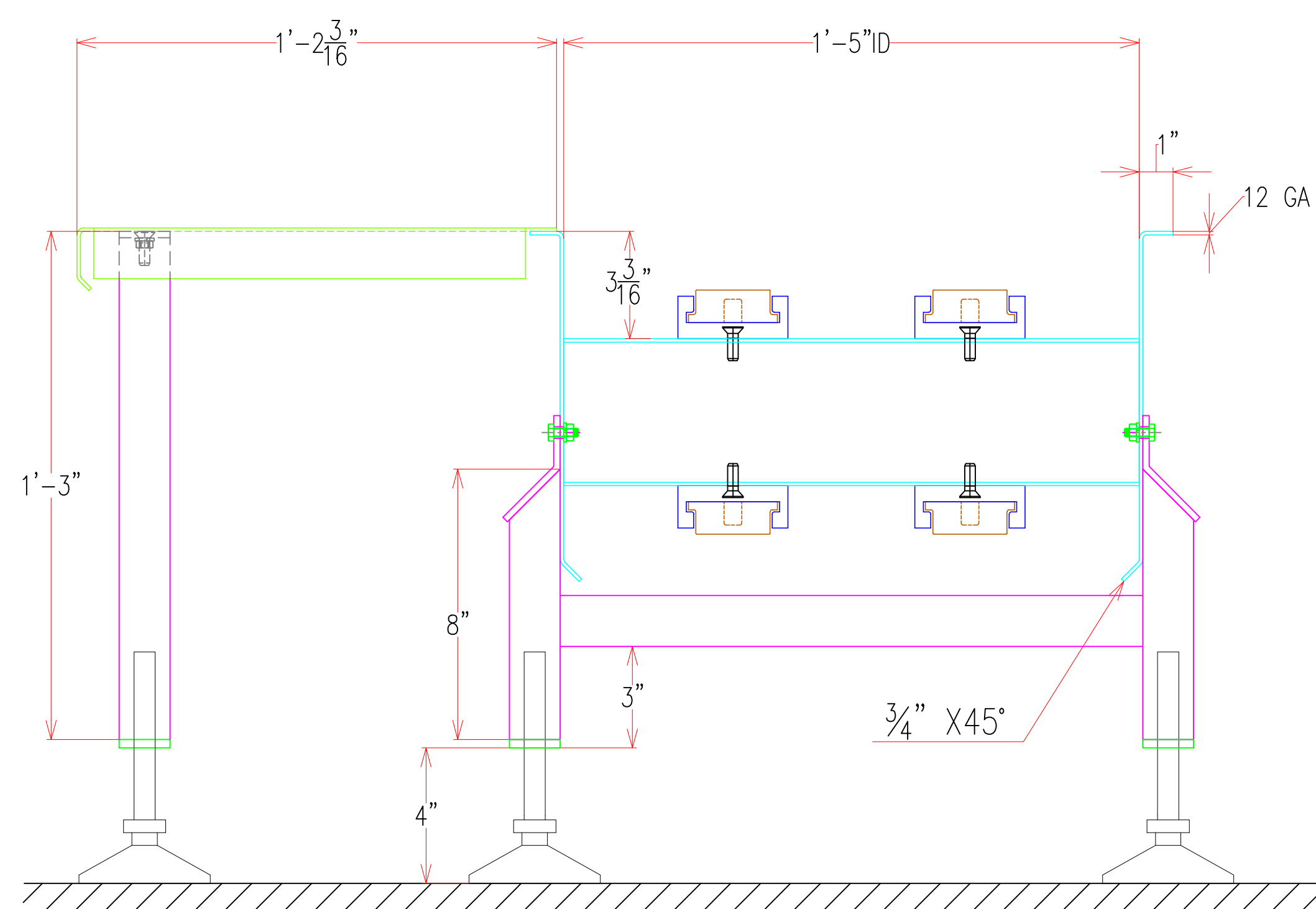
CROSS SECTION
